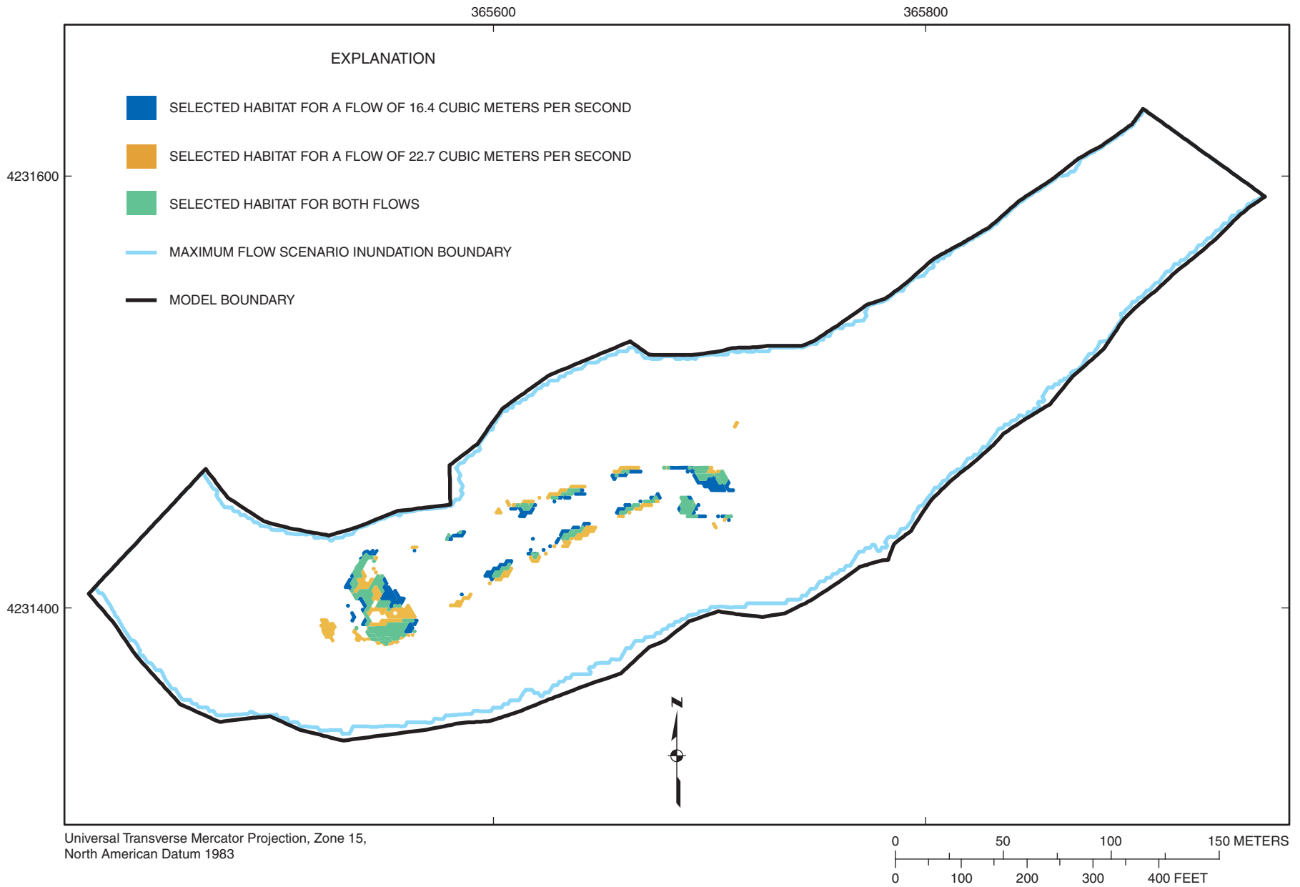
Figure 4-62. Selected habitat area distribution for habitat categories 16, 17 combined (channel catfish) at flows of 16.4 and 22.7 cubic meters per second at Marais des Cygnes River site MDC2.
